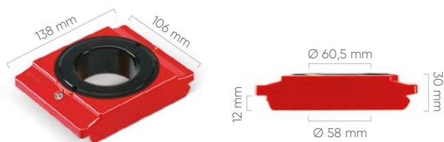
TOOL HOLDER HSK A80-B100
