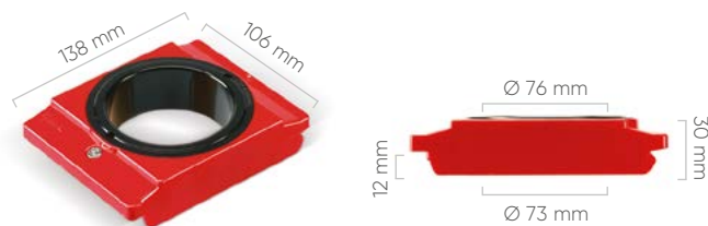
TOOL HOLDER HSK A100-B125
