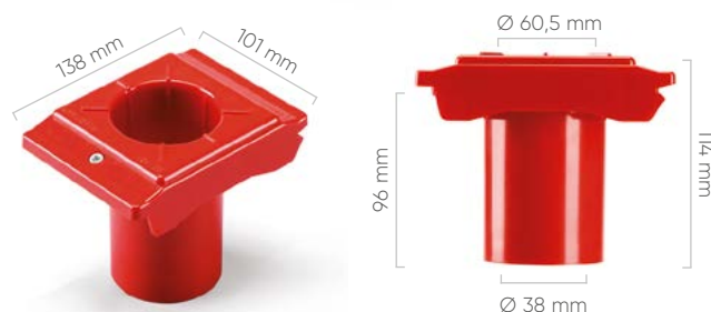
TOOL HOLDER VDI 60
