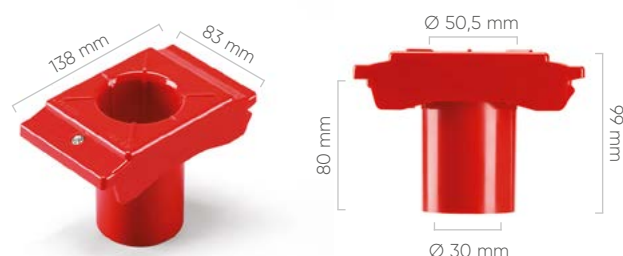
TOOL HOLDER VDI 50
