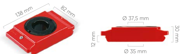
TOOL HOLDER HSK A50-B63
