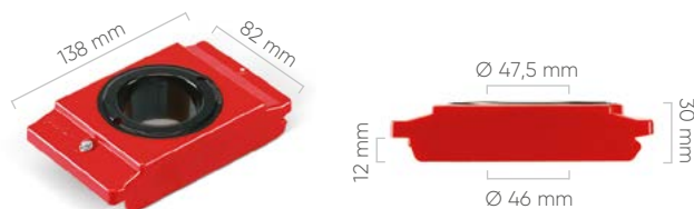
TOOL HOLDER HSK A63-B80
