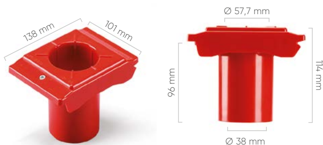
TOOL HOLDER 2" 1/4
