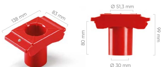
TOOL HOLDER 2"
